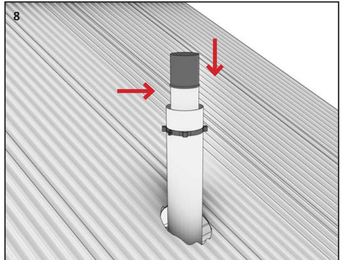
Trim the 150mm Ø flue to the required total flue height and lower onto the already installed flue. Seal and rivet in place. Fit the 200-250mm spacer onto the 200mm Ø liner.
