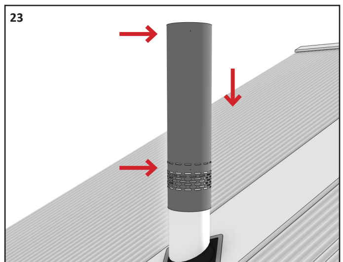
Lower the Upper Designer Shroud over the flue cowl and cone. The top of the Designer Shroud MUST line up with the top of the cowl. Screw fix to the cowl and cone.
