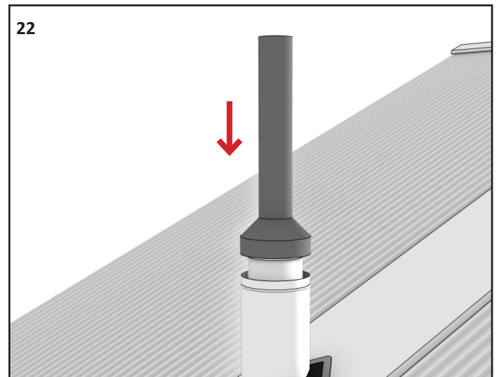
Slide the cone/casing cover over the 150mm Ø flue until it stops at the spider bracket.
