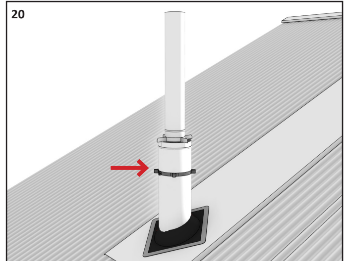
Installing the Designer Flue Shroud involves a few extra steps. Before fitting the cone and cowl, Fit the 250-320mm spider bracket onto the onto the lower 250mm Ø liner.
