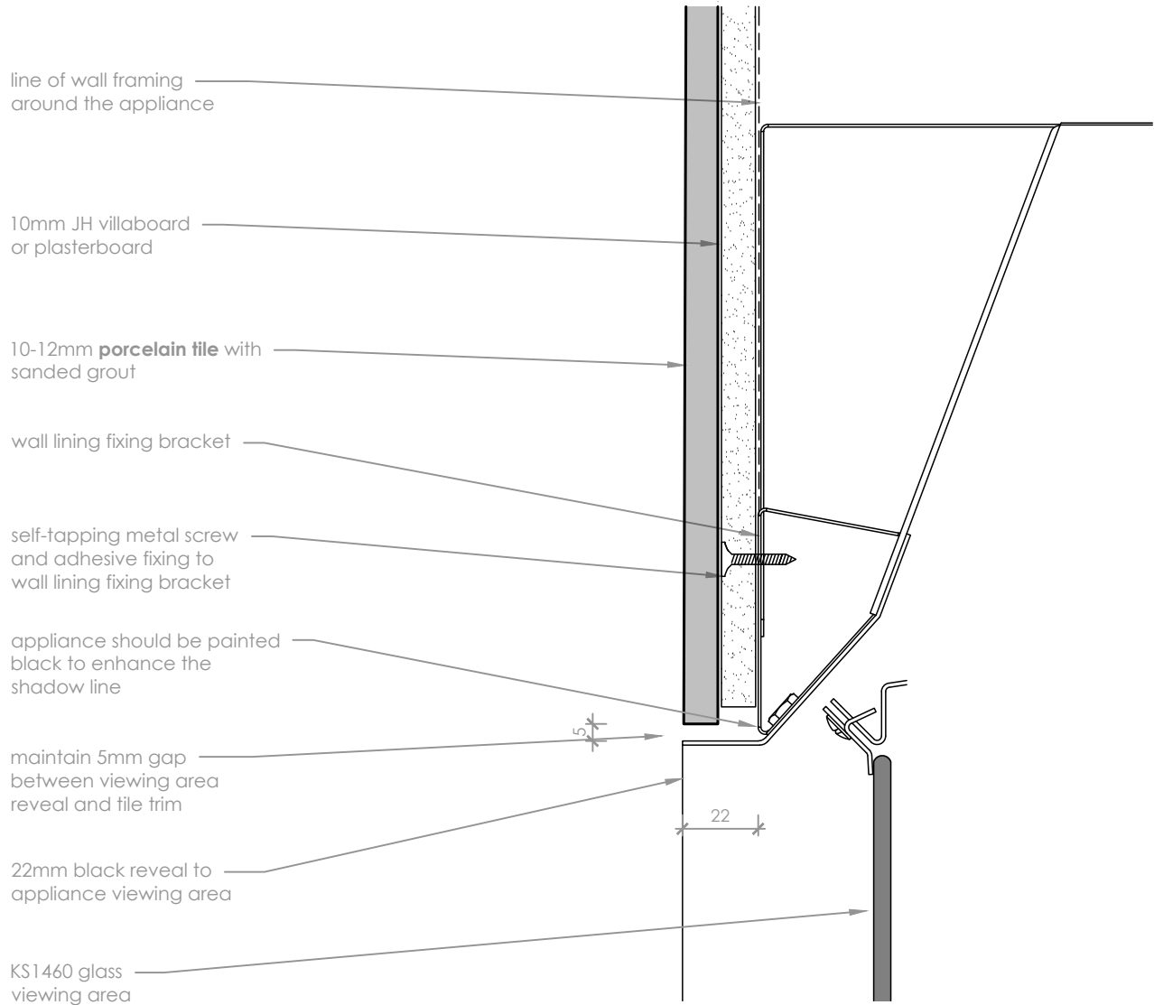
Tile Detail
